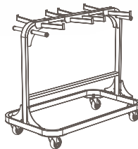
LEG TRANSFER AND STORAGE CART L55.5" W31" H50" L141cm W79cm H127.5cm holds up to 16 folded CliX legs
