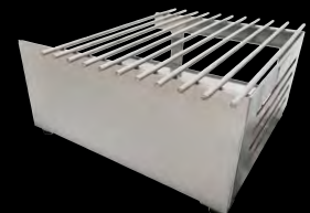
CVR Butane Stove Cover CM-CVR L 14.25" (362 mm) W 12" (305 mm) H 7.2" (183 mm)
